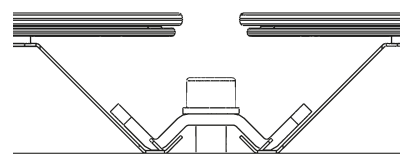
Fig. 3 Mounting of a SMART clamp
